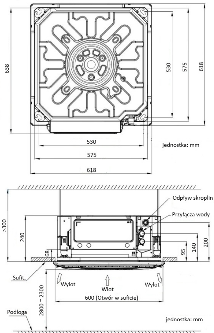
SF2-300C2 / SF2-400C2 / SF2-500C2
