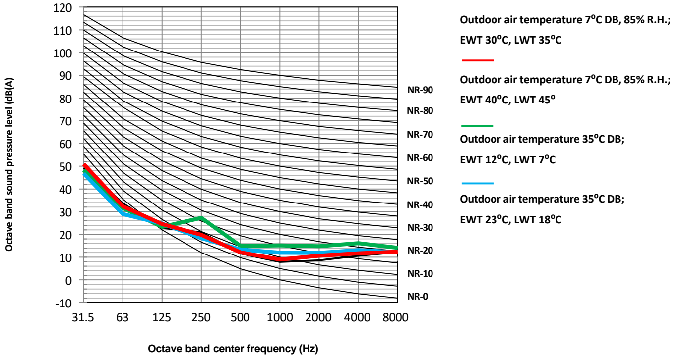
MSH-40EB + MSH-190TB/3 octave band levels
