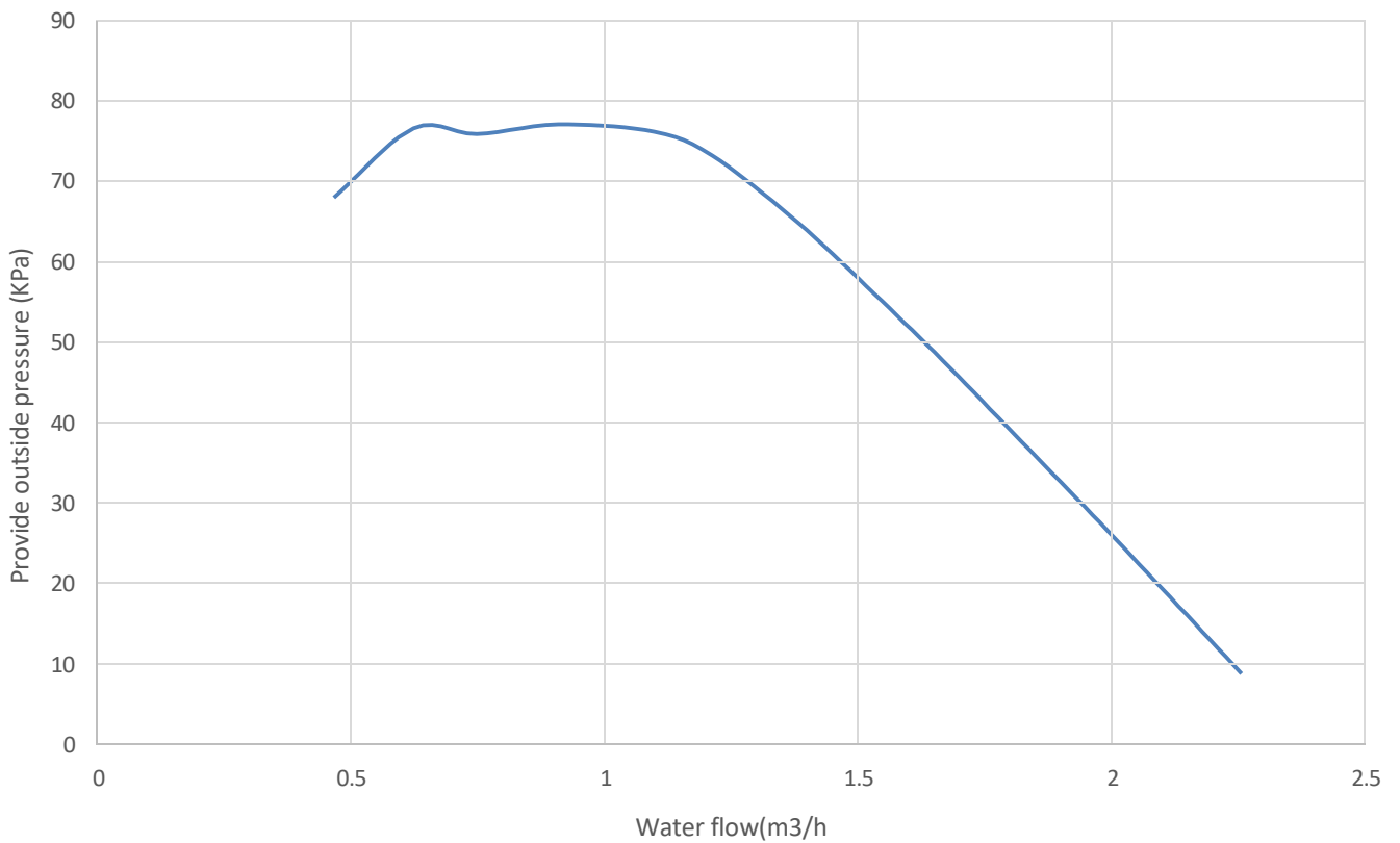
Hydro module with 240L water tank
