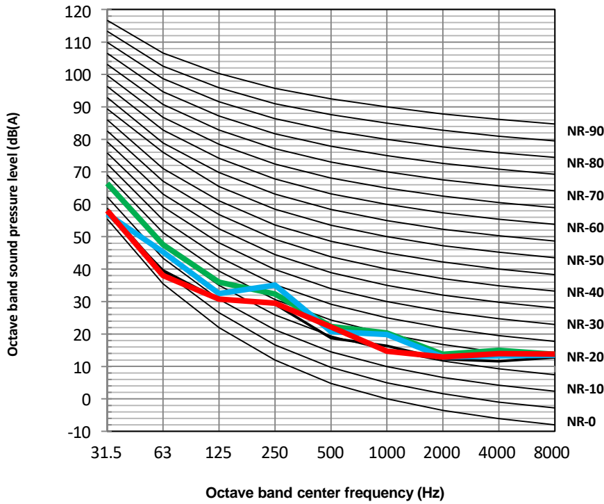
MSH-140EB-3 + MSH-240TB-3/9 octave band levels
