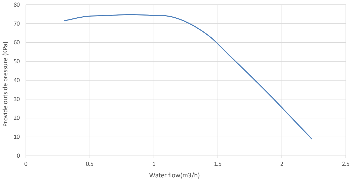
Hydro module with 240L water tank
