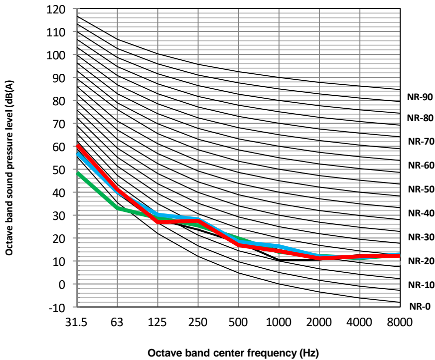
MSH-120EB-3 + MSH-240TB-3/9 octave band levels
