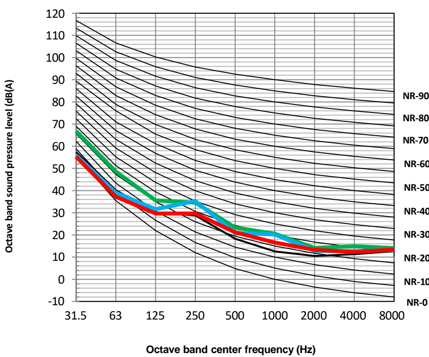
MSH-160EB-3 + MSH-240TB-3/9 octave band levels
