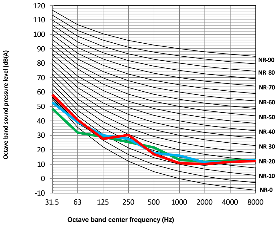
MSH-80EB + MSH-190TB-3/9 octave band levels
