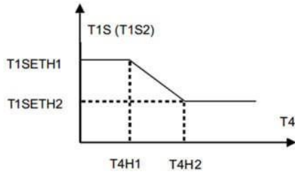
Automatic setting curve for heating mode
