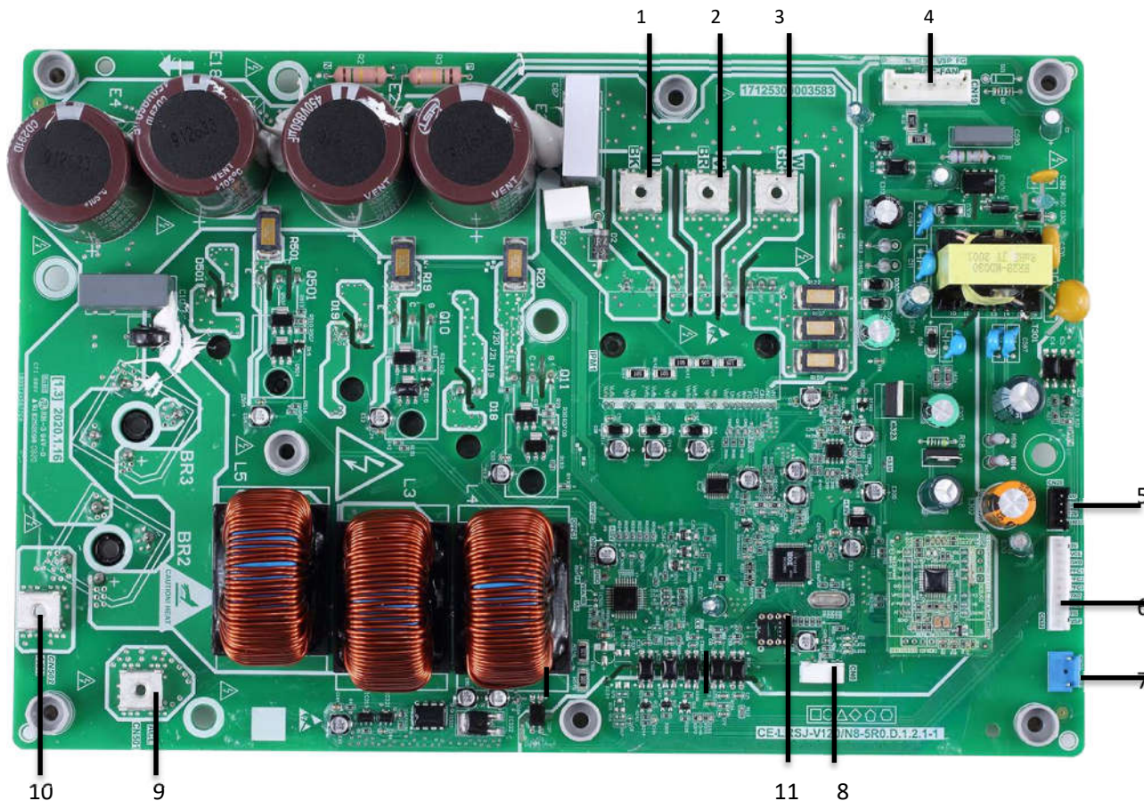
Figure 4-2.6: MSH-120EB; MSH-140EB; MSH-160EB outdoor unit inverter module
