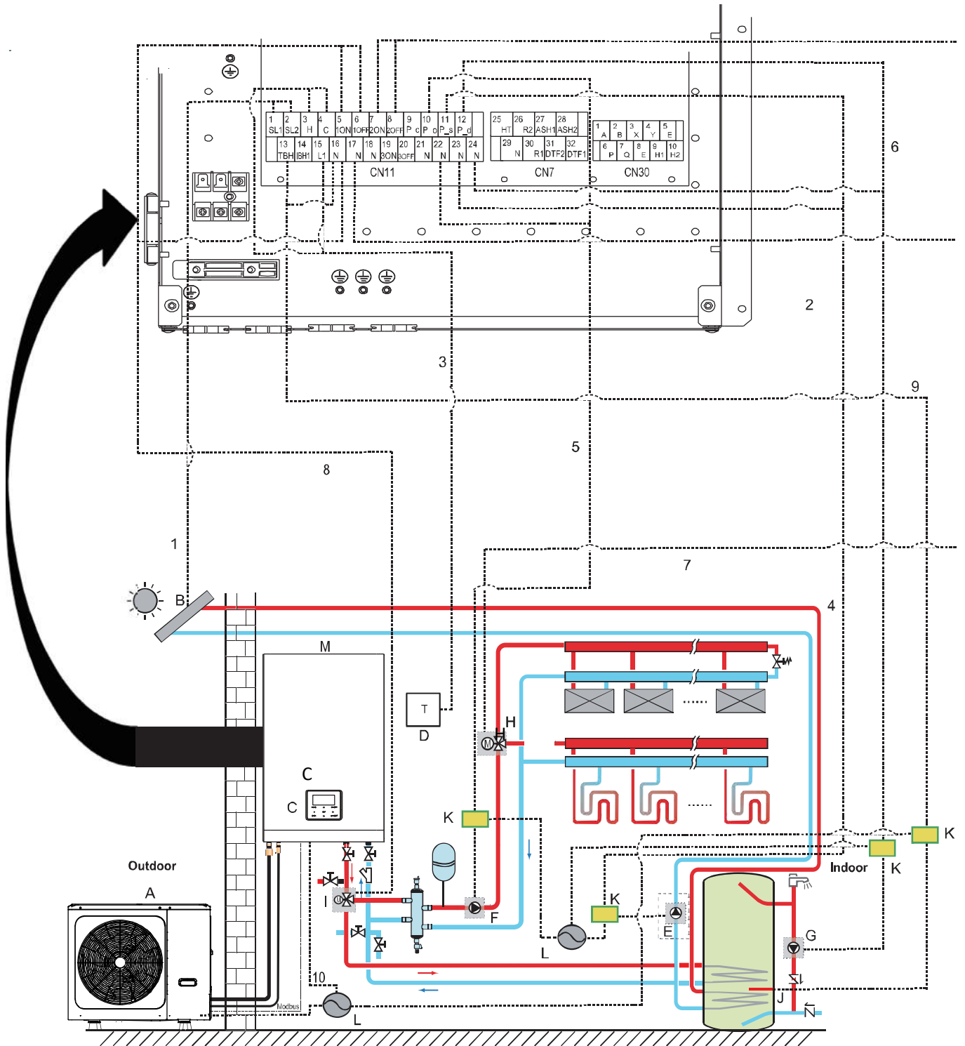
Figure 3-5.1: Wiring overview
