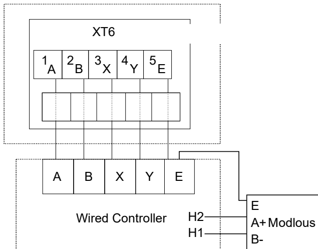
Figure 4-2.12: Wiring
