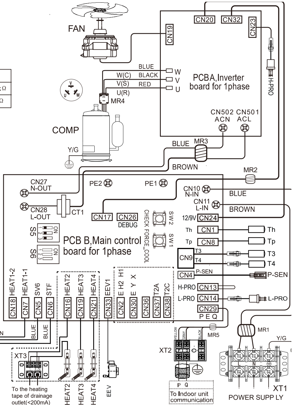
Figure 2-4.1: MSH-120EB; MSH-140EB; MSH-160EB wiring diagram
