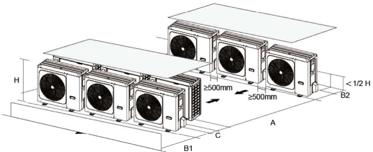
Figure 3-2.11: Multi-row installation
