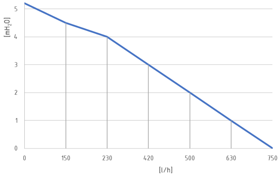
Bypass/circulation pump characteristics.
