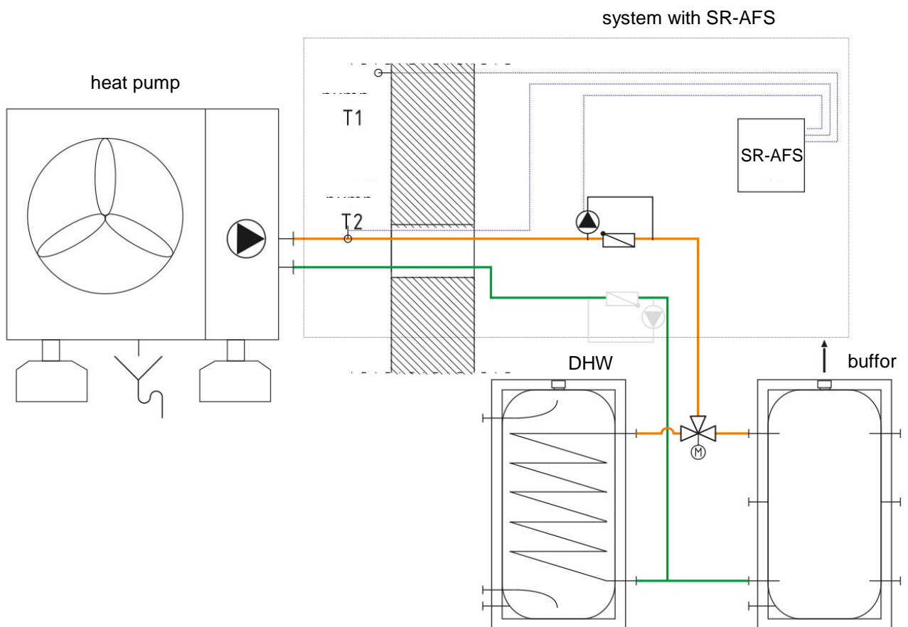
An example of a hydraulic diagram.
