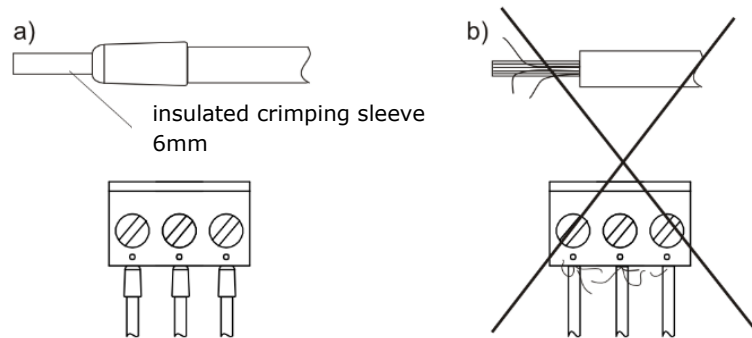
Securing the ends of the wires: a) - correct, b) - incorrect.
